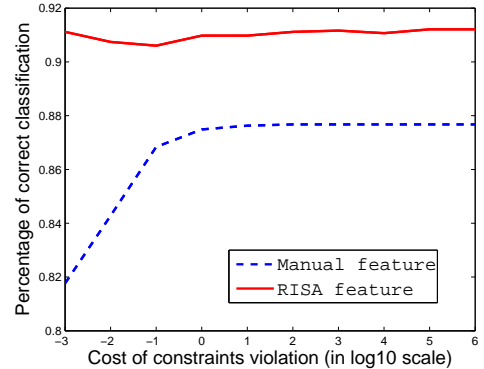
Fig. 5. Performance comparison of features learned from RISA with manually selection features. The classification performance was evaluated based on L2-regularized L2-loss support vector classification implemented through LibLINEAR Library. The plot is a sensitivity analysis for the regularization term, along the X axis, which controls the trade off between regularization and correct classification within the SVM framework.
