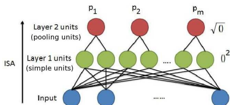
Fig. 2. The neural network architecture of an ISA network. The red bubbles are the pooling units whereas the green bubbles are the simple units. In this picture, the size of the subspace is 2: each red pooling unit looks at 2 simple units.
